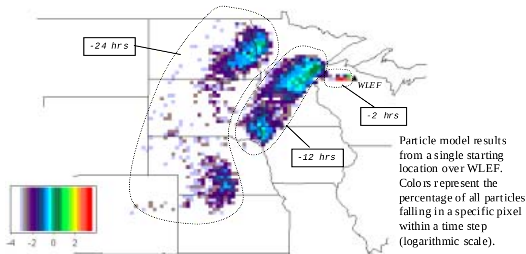
(a) Backward Particle Dispersion Results: 990608 UT1300 1000 AGL
