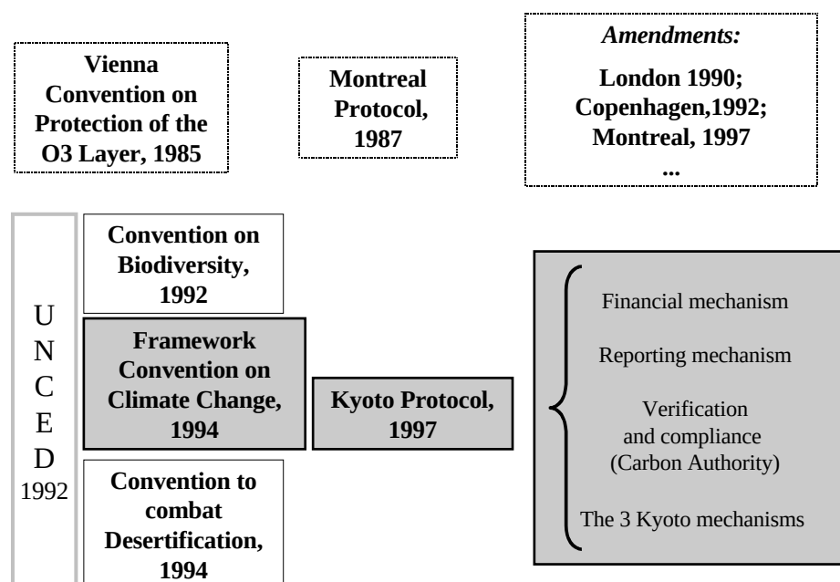
Figure 1: overview of the three “Rio Conventions”, together with the Montreal Protocol to reduce the substances that deplete the ozone layer. The Rio Conventions derive from the United Nations Conference on Environment and Development (UNCED) held at Rio, Brazil, in 1992
