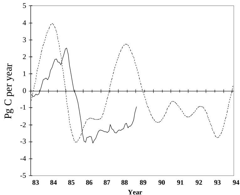
Figure 1. NASA-CASA model estimate (solid line) of global ecosystem carbon exchange with the atmosphere, compared to terrestrial biosphere flux of carbon recomputed from isotopic ( \delta^{13}\text{C} ) deconvolution data (Keeling et al. , 1995; dashed line). Running 12-month totals are plotted. Positive yearly mean values represent a net source flux from the biosphere to the atmosphere, whereas negative yearly values represent a net sink flux into the biosphere from the atmosphere.
