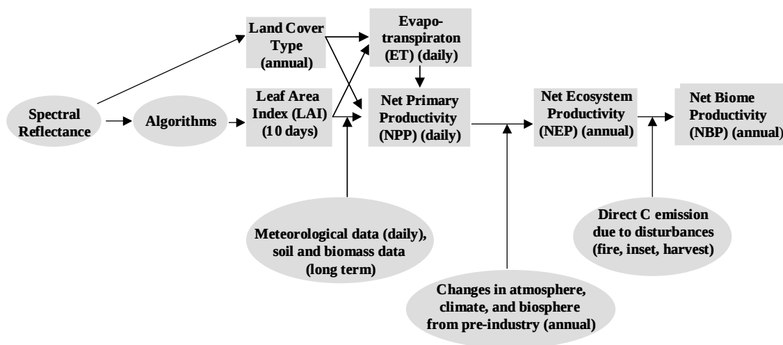
Figure A1. The major steps to use satellite spectral measurements for terrestrial carbon cycle estimation. The major ancillary data required at each step are also included.
